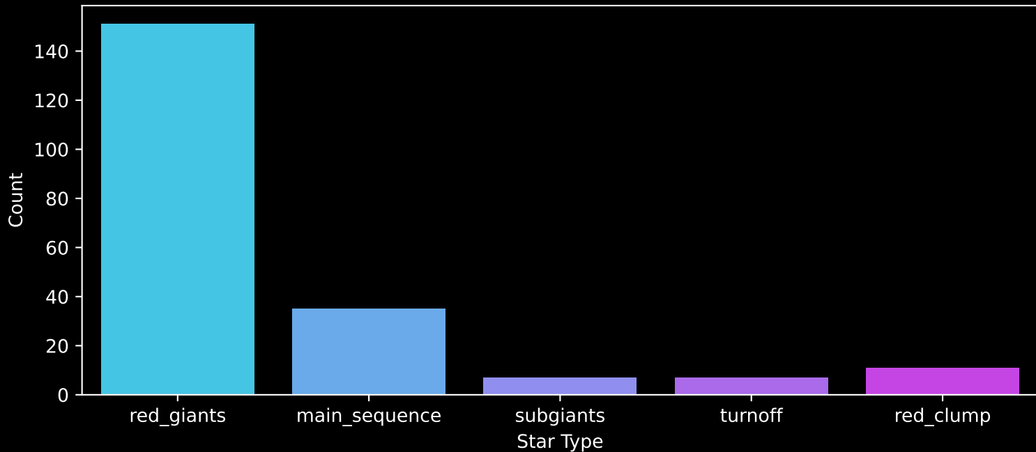
APOGEE DR17 Field: [Berkeley75] Count plot of Star Type
