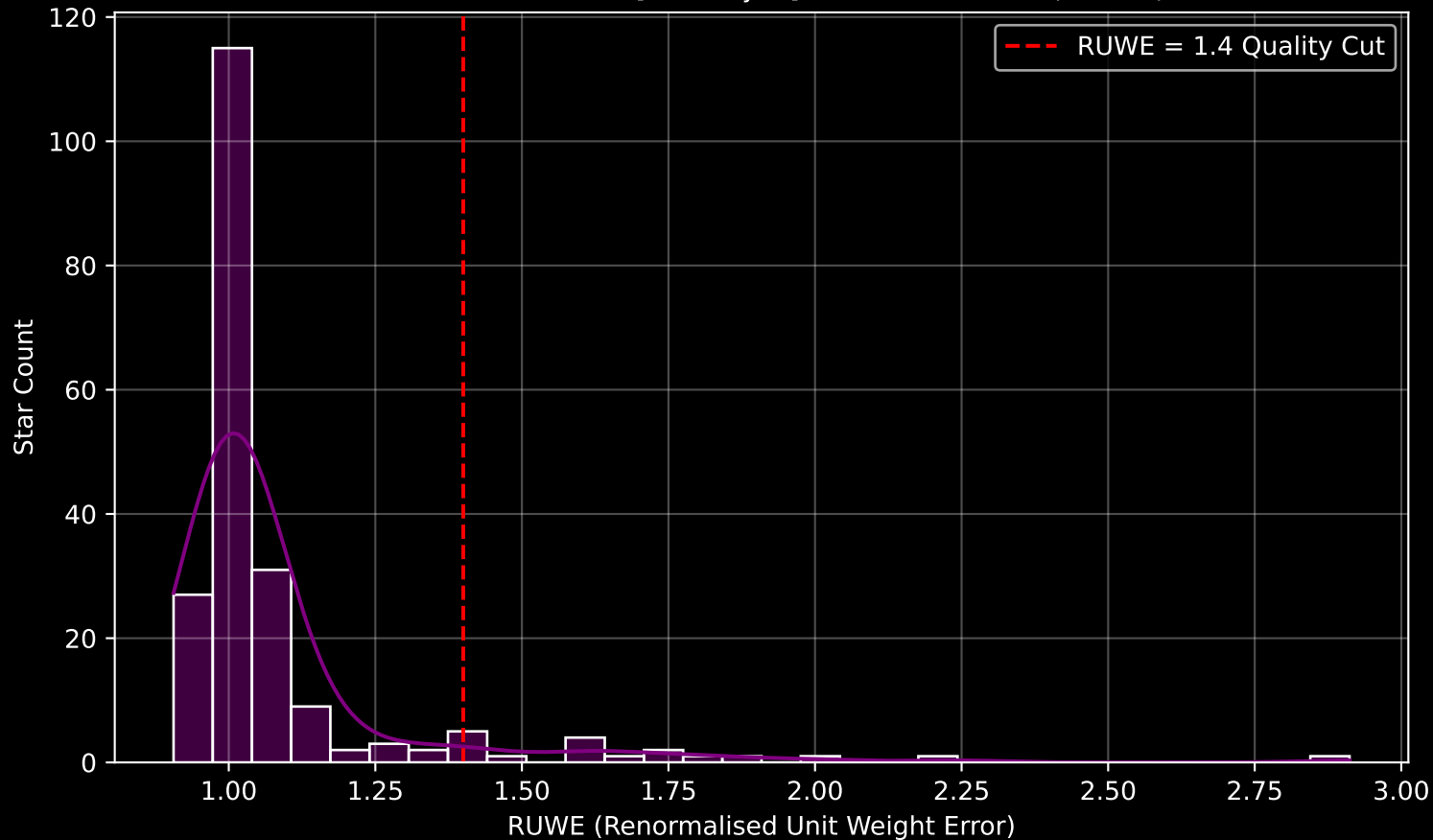
GAPOGEE DR17 Field [Berkeley75] RUWE Distribution (n= 207)
