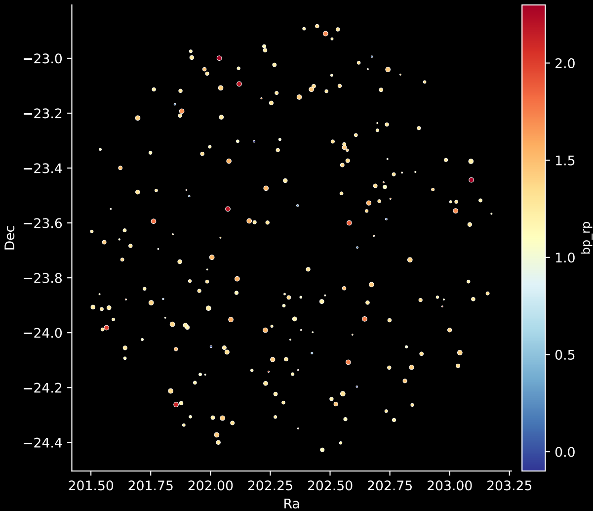
APOGEE DR17 Field: [Berkeley75] Stars: 211
