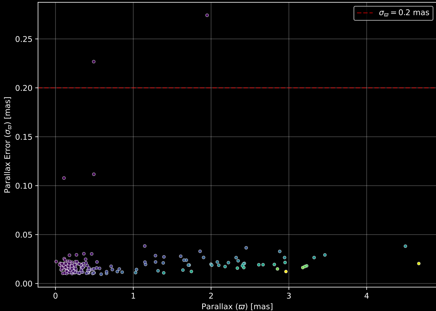
APOGEE DR17 Field: [Berkeley75] Parallax Quality (n= 211)
