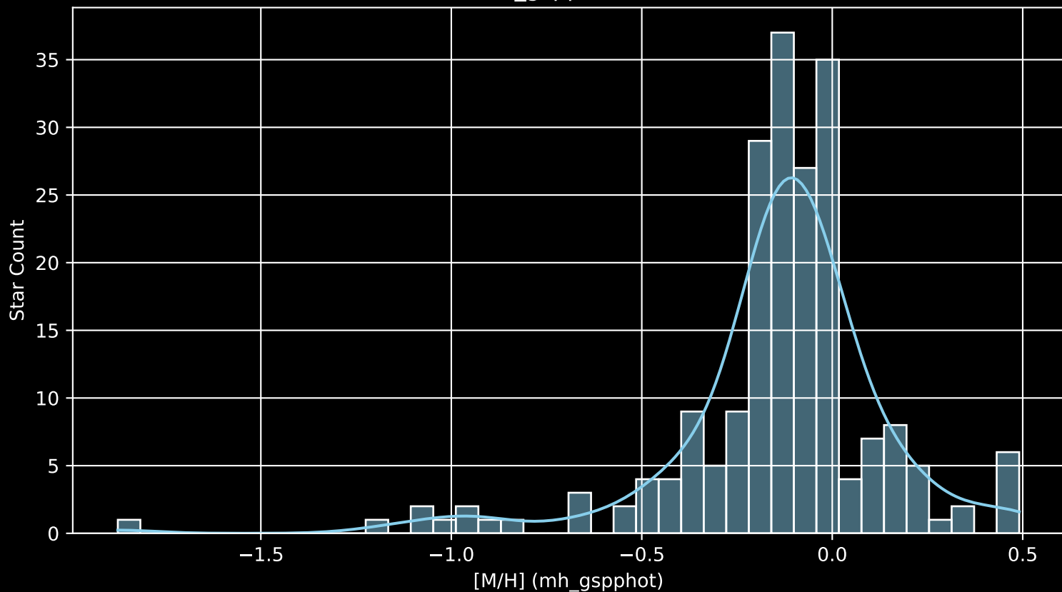
APOGEE DR17 Field: [Berkeley75 [M/H] (mh_gspphot) (n= 206)
