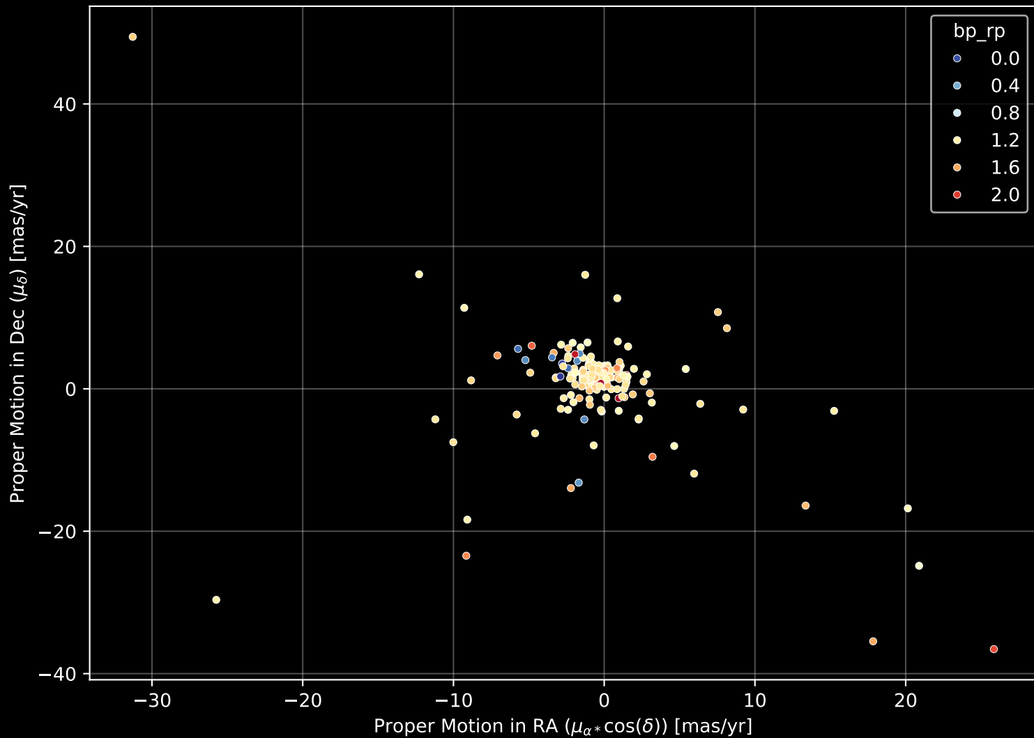
APOGEE DR17 Field: [Berkeley75] Proper Motion Diagram (n= 211)
